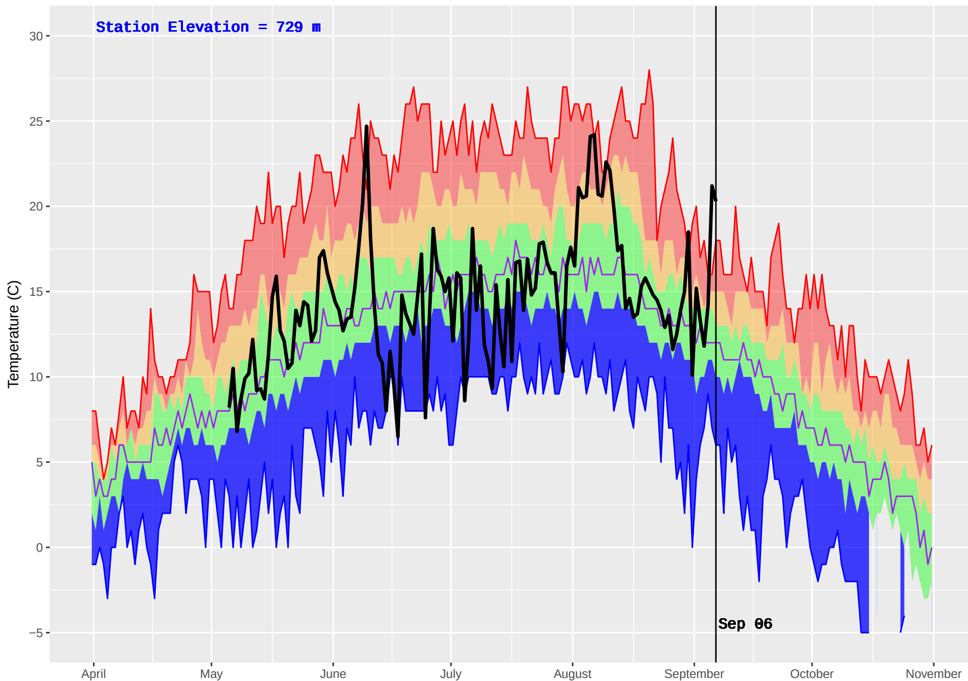
ATLIN (111) : Historical (1977–2016) and Current (2017) Noon Temperature
