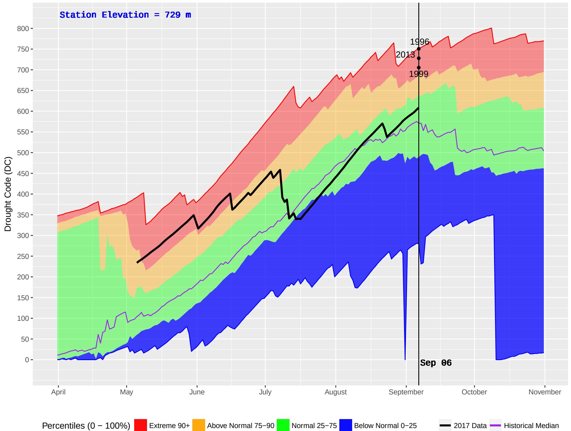
ATLIN (111) : Historical (1977–2016) and Current (2017) Noon Drought Code (DC)
