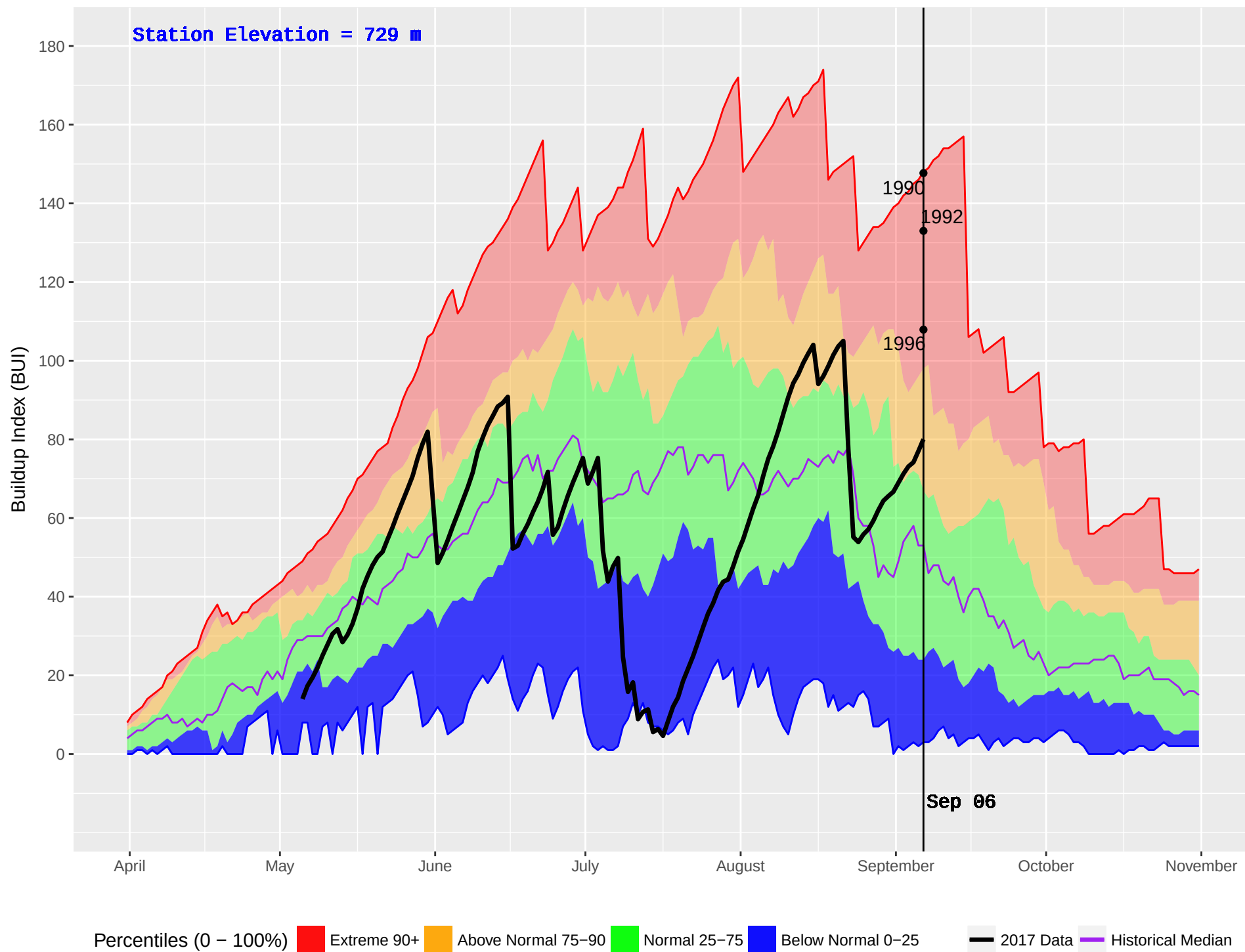
ATLIN (111) : Historical (1977–2016) and Current (2017) Noon Buildup Index (BUI)
