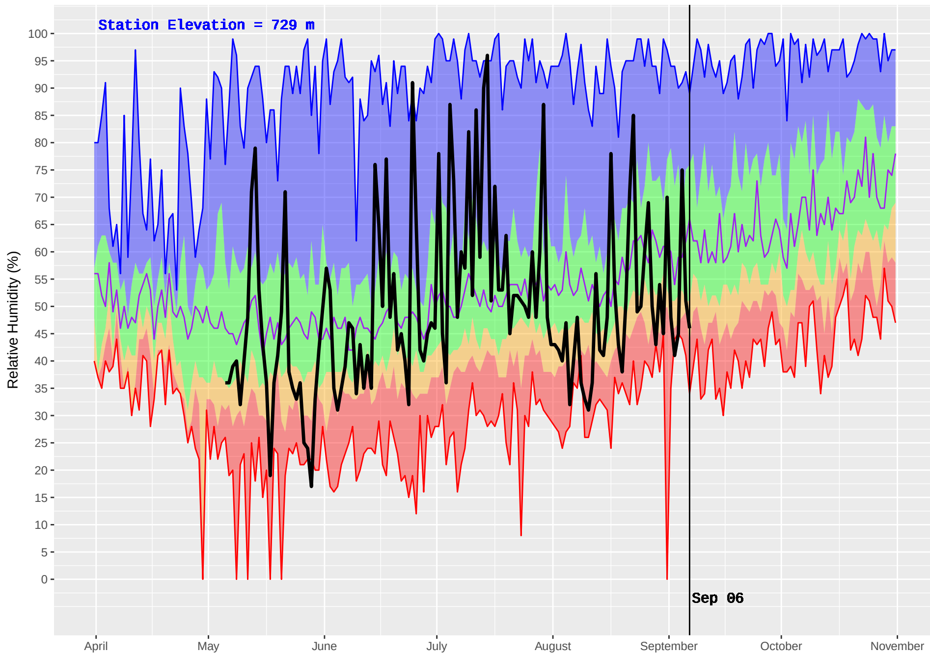
ATLIN (111) : Historical (1977–2016) and Current (2017) Noon Relative Humidity
